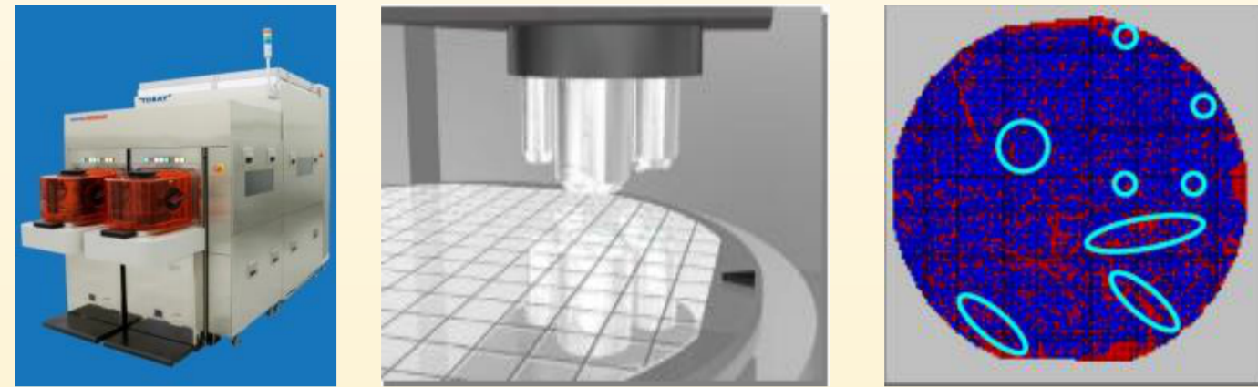
Fully automated inspection tools for Visual, Infrared and Photoluminescence Inspection
