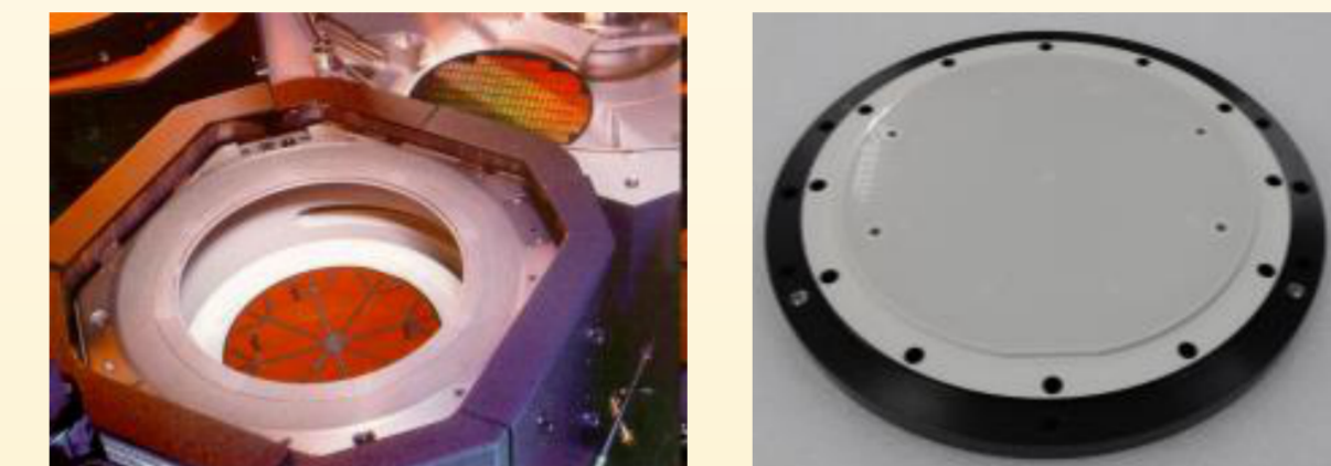
Quartz, Silicon and Ceramic Parts for Plasma Etch and CVD Ceramic Sprayed Electro Static Chucks
